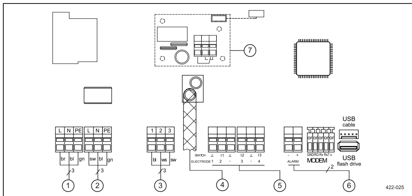
Fig.: Mono connection diagram
