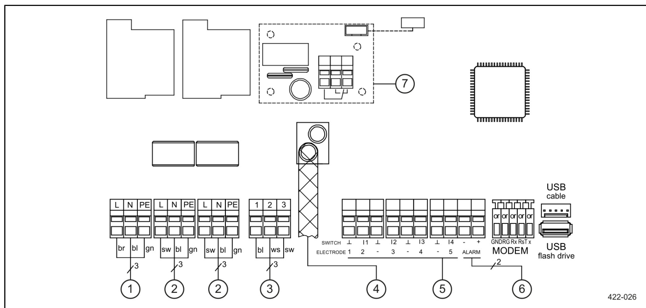
Fig.: Duo connection diagram
