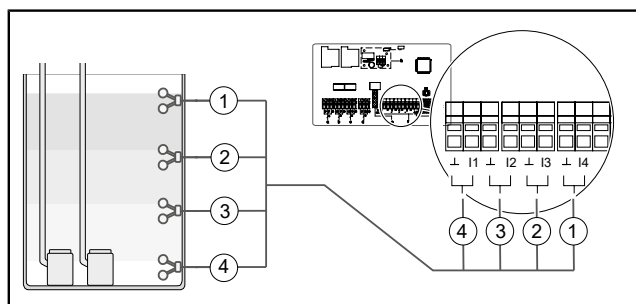
Fig. 1: Float switches Duo
